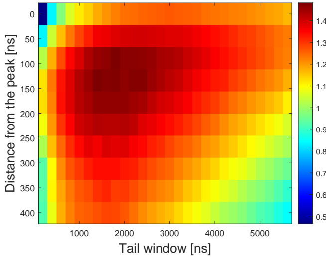
Fig. 7. Variation of the FOM, as a function of the PSD parameters t_s (“distance from the peak”) and t_w (“tail window”), as used in eq. (4). The FOM was calculated, for every set of parameters, by means of eq. (5).
