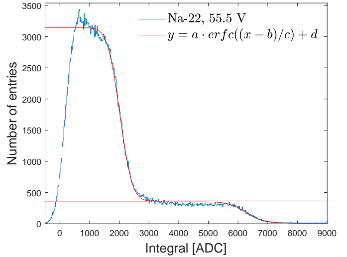
Fig. 1. Energy spectrum of the ^{22}\text{Na} source, obtained at 55.5 V (4 V above the breakdown voltage) and shown altogether with the error function fitted to the Compton edge.
