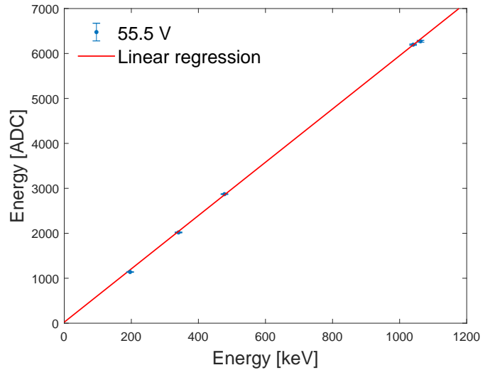
Fig. 2. Calibration line at 55.5 V (4 V above the breakdown voltage), obtained by using the sources reported in Table III.
