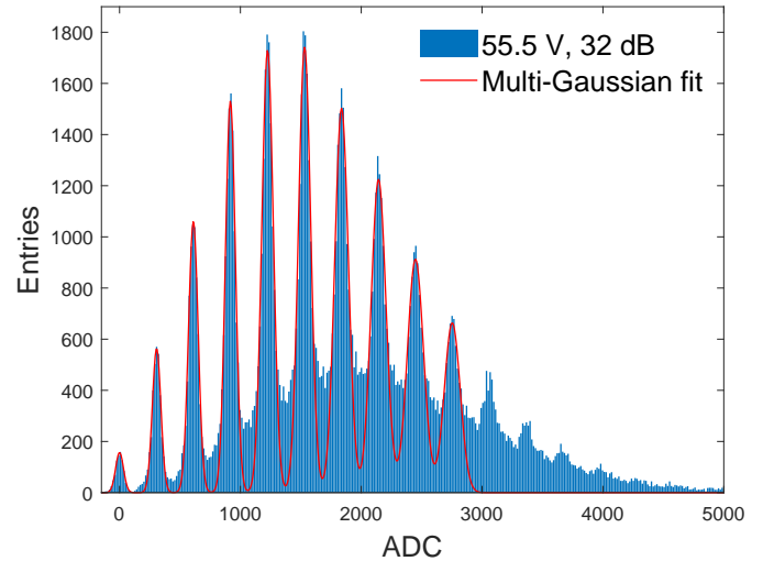
Fig. 3. Frequency histogram of the integrals of the signals (multi-photon spectrum) obtained at 55.5 V (4 V above the breakdown voltage) and amplification gain 32 dB.
