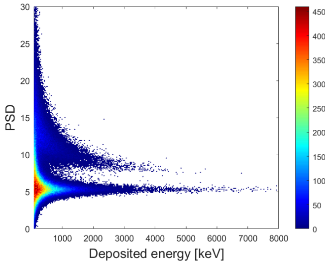
Fig. 8. 2D histogram of the PSD values against the deposited energies recorded with the ^{252}\text{Cf} source, biasing the SiPM at 55.5 V (4 V above the breakdown voltage). The deposited energies results by the calibration coefficients as of section II-A. The upper branch of the plot represents neutron detection.
