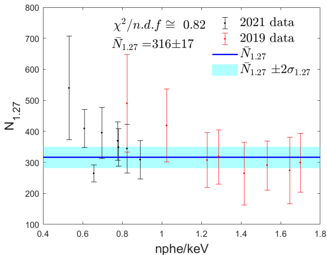
Fig. 14. Minimum number of detected photons ( N_{1.27} ) required to reach FOM = 1.27 shown as a function of the system sensitivity (in terms of p.e./keV). The labels “2021 data” “2019 data” are used in the same sense of Fig. 13. The blue line corresponds to the weighted mean and the \chi^2 value shows a fair agreement with the hypothesis of having a constant N_{1.27} as the operational conditions are changed.
