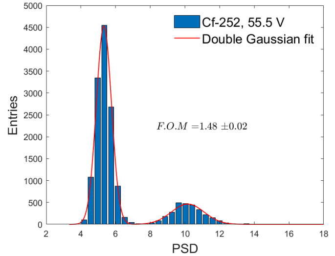
Fig. 9. Histogram of the PSDs shown in figure 8, obtained by biasing the SiPM at 55.5 V (4 V above the breakdown voltage) and considering only the events with energy E inside the projection window 1 \text{ MeV} \leq E \leq 1.5 \text{ MeV} . The geometric separation between the fitted curves gives the FOM, as indicated in eq. (5).
