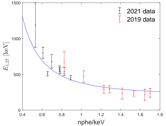
Fig. 13. Minimum energy deposit corresponding to FOM = 1.27 (i.e. E_{1.27} ) shown as a function of the number of photoelectrons extracted per keV of energy deposit. The label “2021 data” refer to the first data set analyzed in the article, i.e., the one with an EJ-276 bar without ageing effects. The label “2019 data” refers to the higher light yield data set. The line is simply meant to guide the eye.
