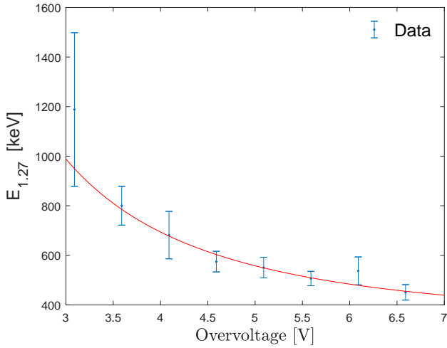
Fig. 11. Minimum energy necessary to reach FOM = 1.27 as a function of the over-voltage applied to sensor. The line is simply meant to guide the eye.
